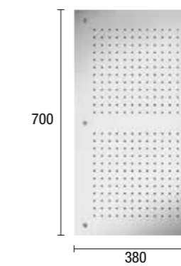
RECTANGULAR TEMPTATION SHOWER HEAD BUILT-IN - STAINLESS STEEL E044088
