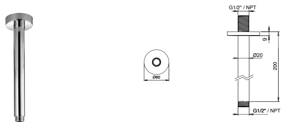
E021018 ROUND ARM WITH ROUND ROSE - BRASS
