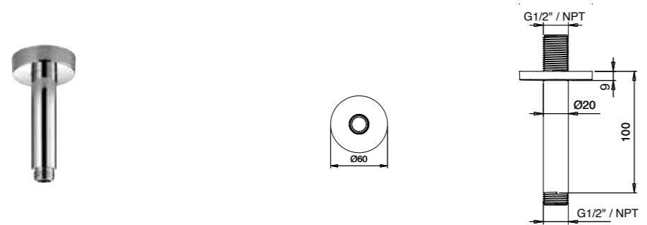
E021017 ROUND ARM WITH ROUND ROSE - BRASS
