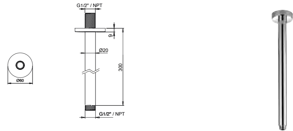
ROUND ARM WITH ROUND ROSE - BRASS E021019
